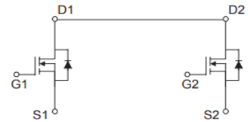
Schematic Diagram
